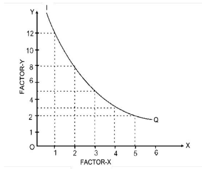
Fig. 2 : Equal Product Curve or Isoquant
